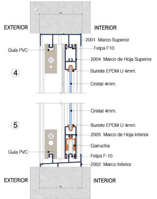
CORTE VERTICAL
