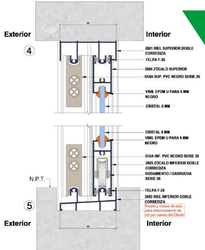
CORTE VERTICAL
