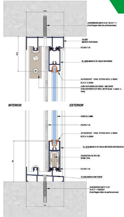
CORTE VERTICAL
