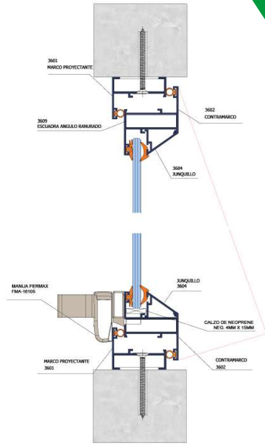
CORTE VERTICAL
